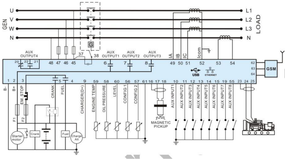
HGM9610 typical application diagram
